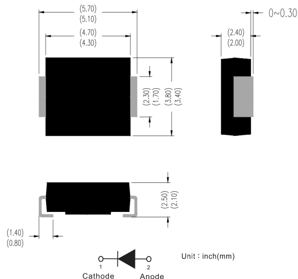
SMB/DO-214AA
